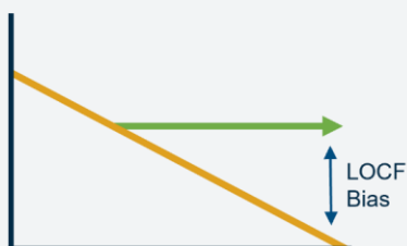
Abb. 6 Imputation mittels LOCF
