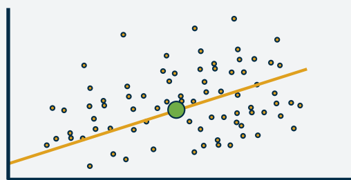
Abb. 4 Imputation via Regression.
